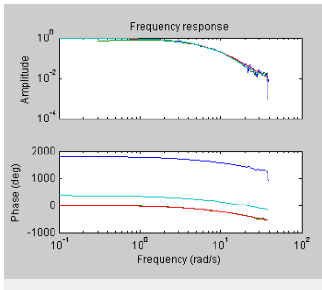
Frequency Response for Models spad, arxqs, and n4s3
