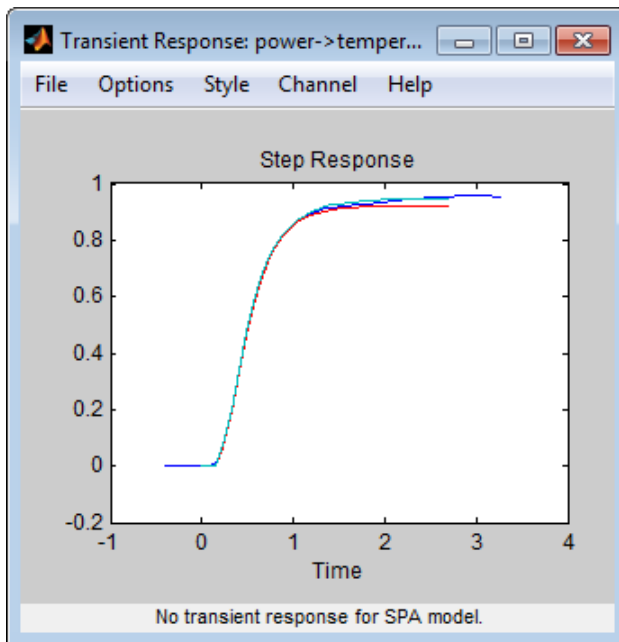
Step Response for imp, arxqs, and n4s3
